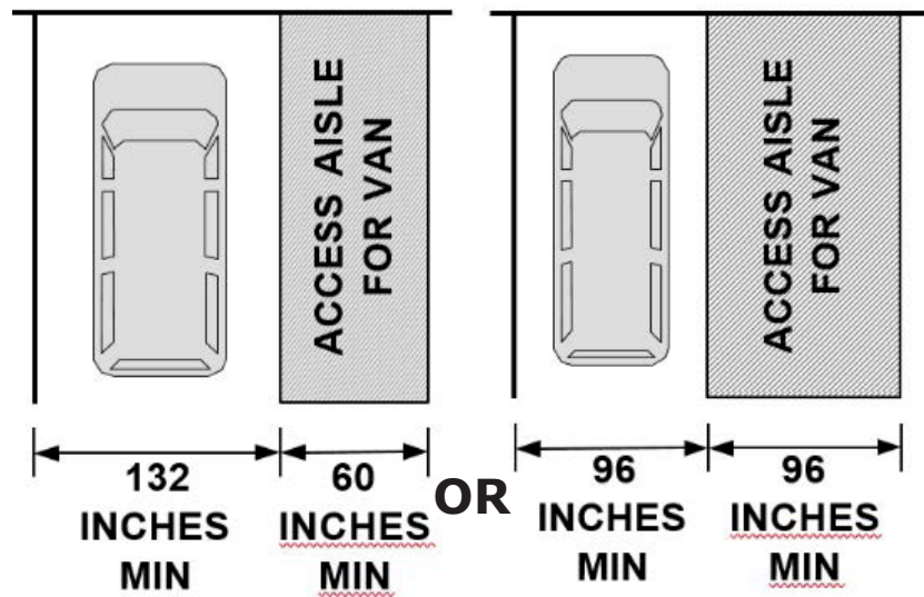
Figure 2: Access aisle
