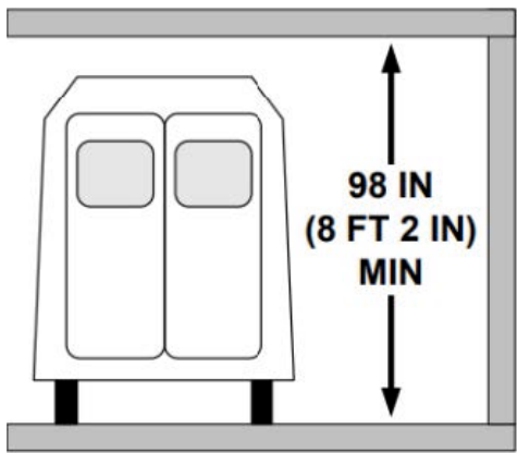
Figure 1: Minimum clearance
